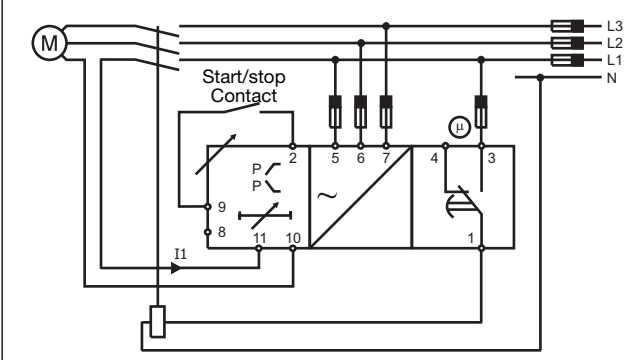
PWB02 - Direct connection - Manual start and stop (NE relay)
