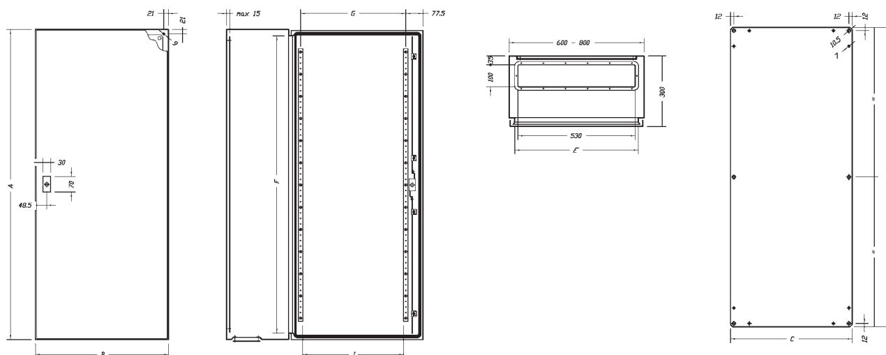
boxes with rod system
