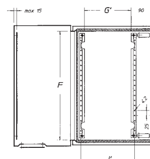
section X - X with open door
