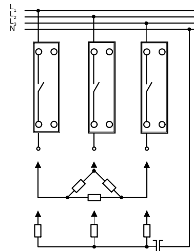
3 single pole relays in 3-phase application Delta, Star, Star with neutral
