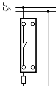
Single pole relay application Line-Neutral, Line-Line
