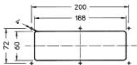
box drilling details
