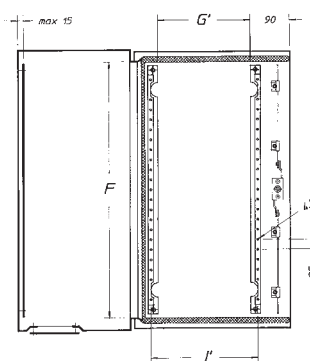
section X - X with open door
