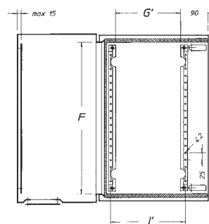
section X - X with open door
