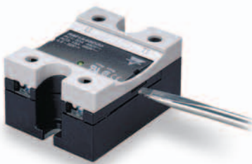
Clip-on protection cover is removable with a screwdriver
