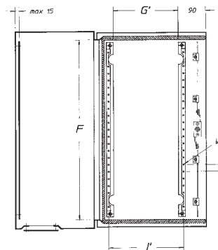
section X - X with open door
