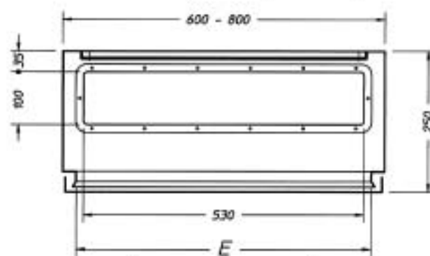
section X - X with open door
