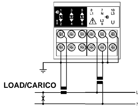
Three-phase input connections - balanced load / Collegamenti ingresso trifase - carico equilibrato
